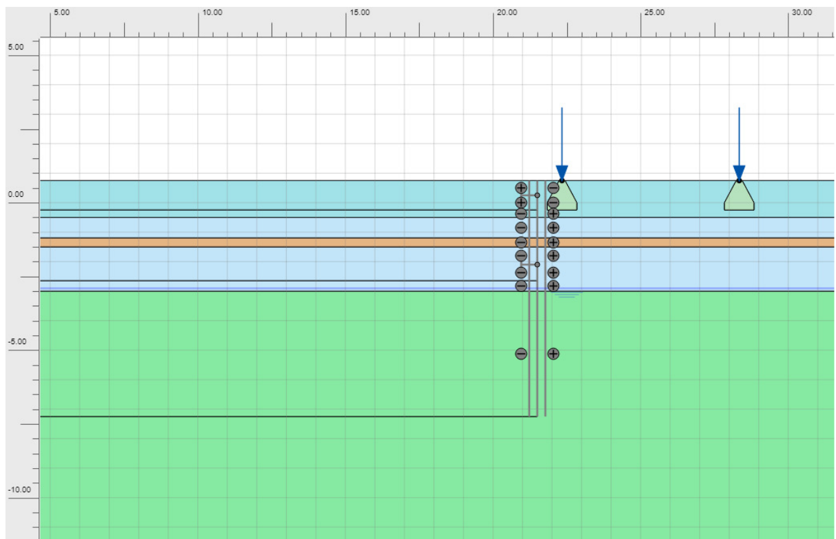
stage 2 - bouwphase belending
